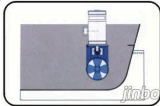
L型传动侧推L-Drive Tunnel Thrusters
