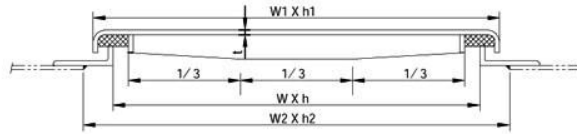
C级圆角钢质门 Level C Round-corner Steel Door
