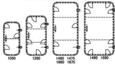
C级圆角带固定圆窗钢质门 Level C Round-corner Steel Door With Fixed Steel Round Window
