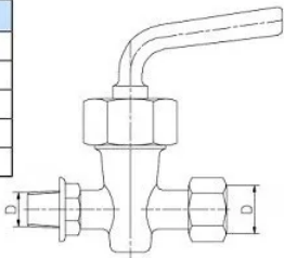
Drain cocks with lever handle male&female ends
