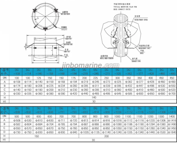
外形尺寸及安装示意 Outline Dimension & Installation Sketch
