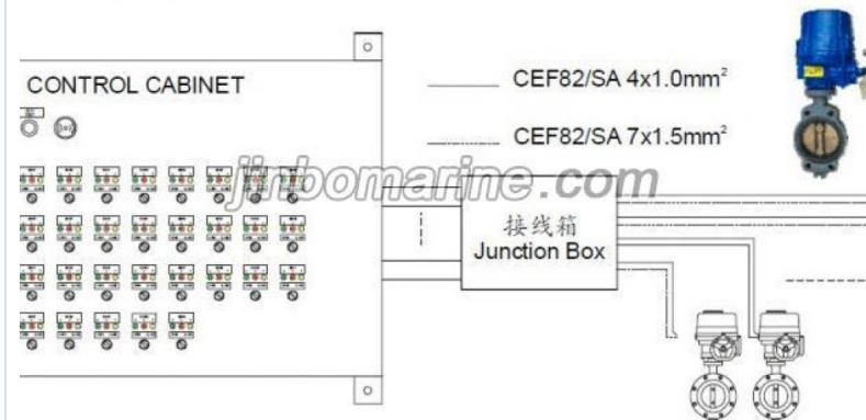
Electric type Valve remote Control System Diagram
