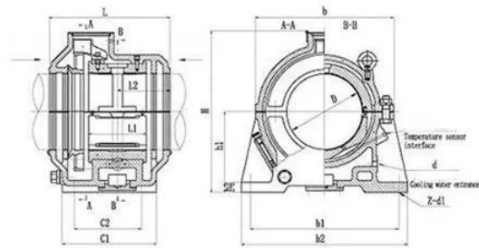
Drawing 3 Type C multi oil wedge gliding intermediate bearing
