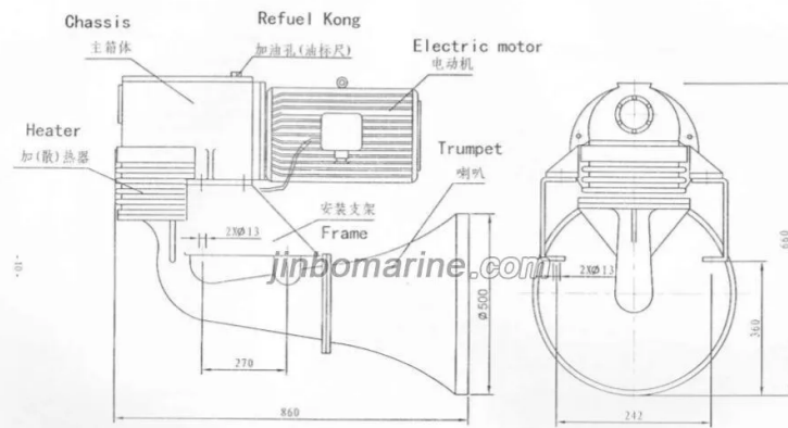
HSD-161型活塞式电动笛外形和安装尺寸 External and Installation Dimension of HSD Whistle
