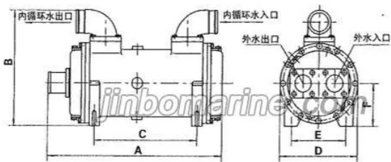
N350, K450 HEAT EXCHANGER
