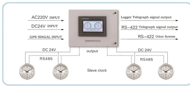
Wiring Diagram of CJCZ-3M II Master-Slave Clock
