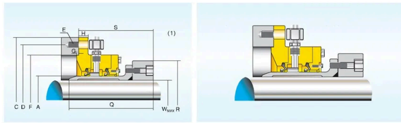
YH3 Oil Lubricated AFT Stern Tube Sealing for Shaft Size 170mm
