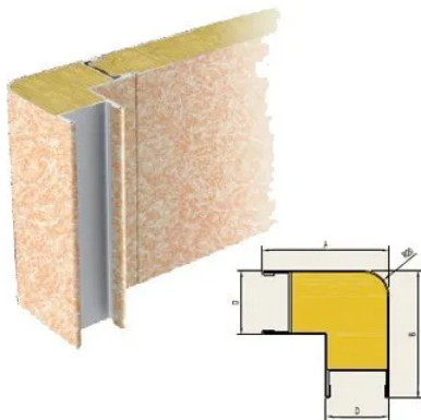
A型圆弧外转角 | Type A External Round Corner
