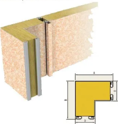
C型外转角 | Type C External Corner
