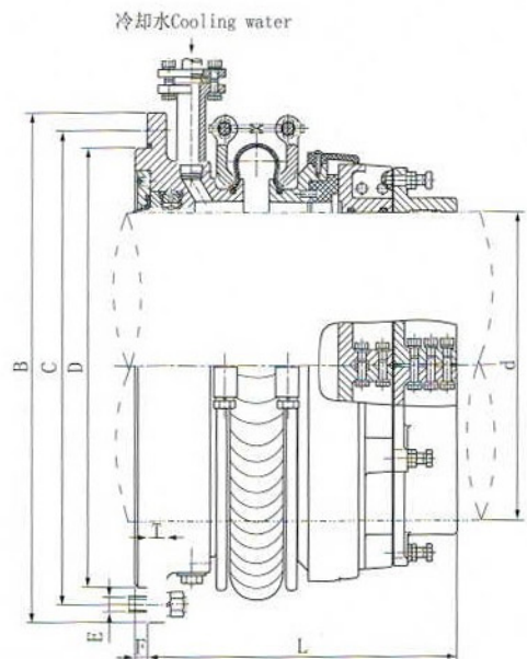
SMA-IIB型水润滑端面密封装置 SMA-IIB water lubrication end face sealing apparatus
