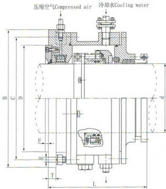
SMA-II型水润滑端面密封装置 SMA-II water lubrication end face sealing apparatus
